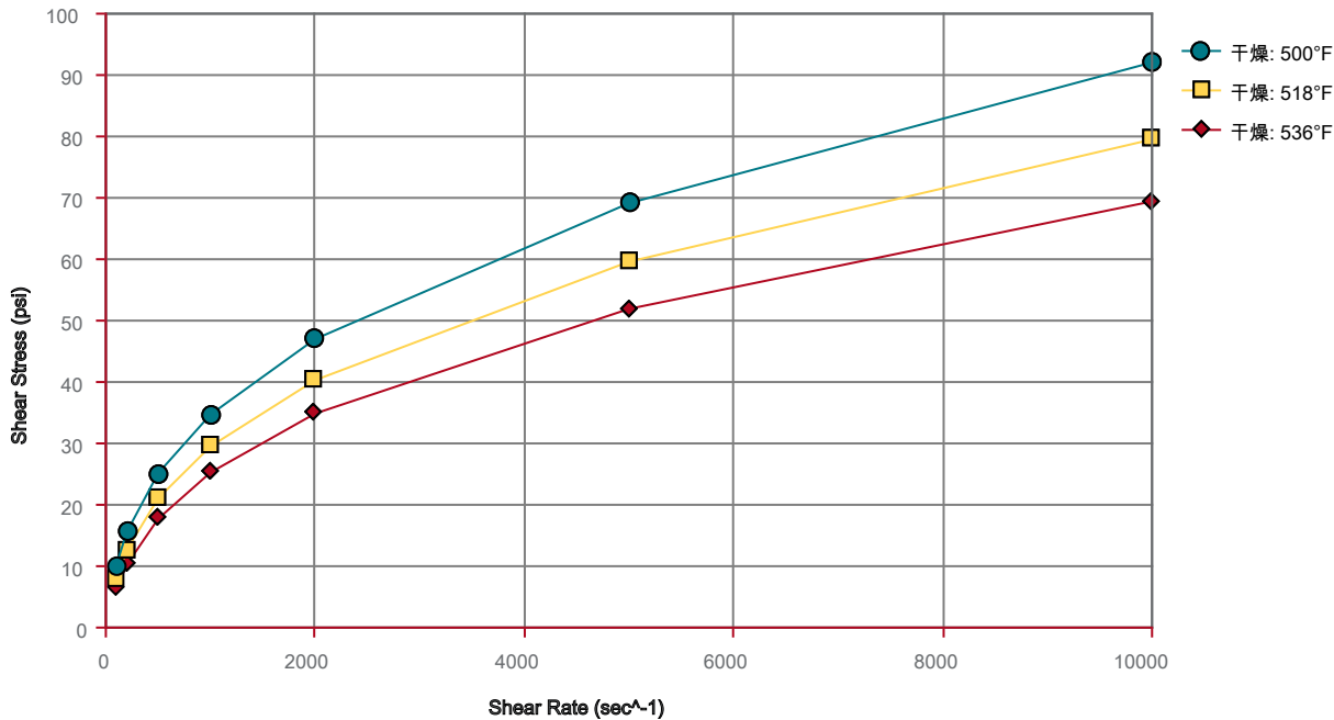
Shear Stress vs. Shear Rate (ISO 11403-1)
